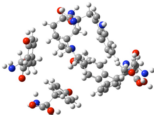
Figure 1: Aromatic box binding site from AChBP (TRP 143, TYR 89, TYR 185, TYR 192, TRP 261) with and without nicotine.
